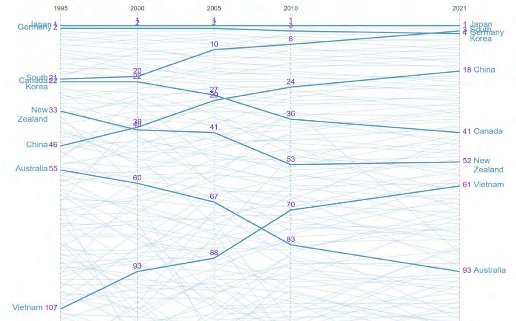
Figure 7: Complexity comparison
