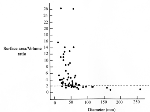
Figure 10A: Surface area to volume ( A/V ) ratio versus diameter (mm) in Dickinsonia fossils of known profile thickness and diameter but assuming that they are composed of tapering cylindrical segments ( n=60 ; based on raw data from Retallack, 2007). Dotted line indicates an A/V ratio of 2.0.
