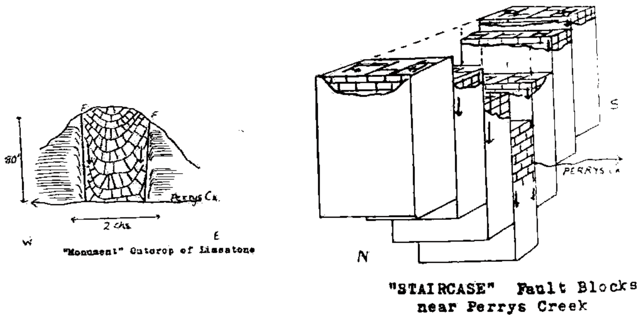
Fig. 6.—Diagrams of the Perry's Creek Step-faulted Trough.
